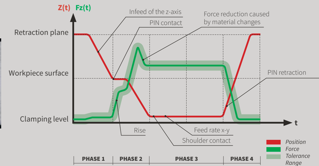
Progression of the pressure force and the position of the tool in the phases of the FSW welding process.
